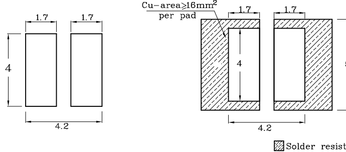
Pad design for improved heat dissipation
